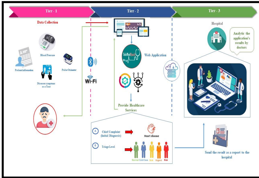
Fig. 3: Proposed Framework
