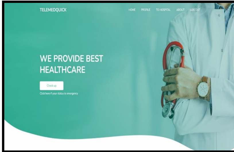
Figure 4: "TeleMedQuick" application
