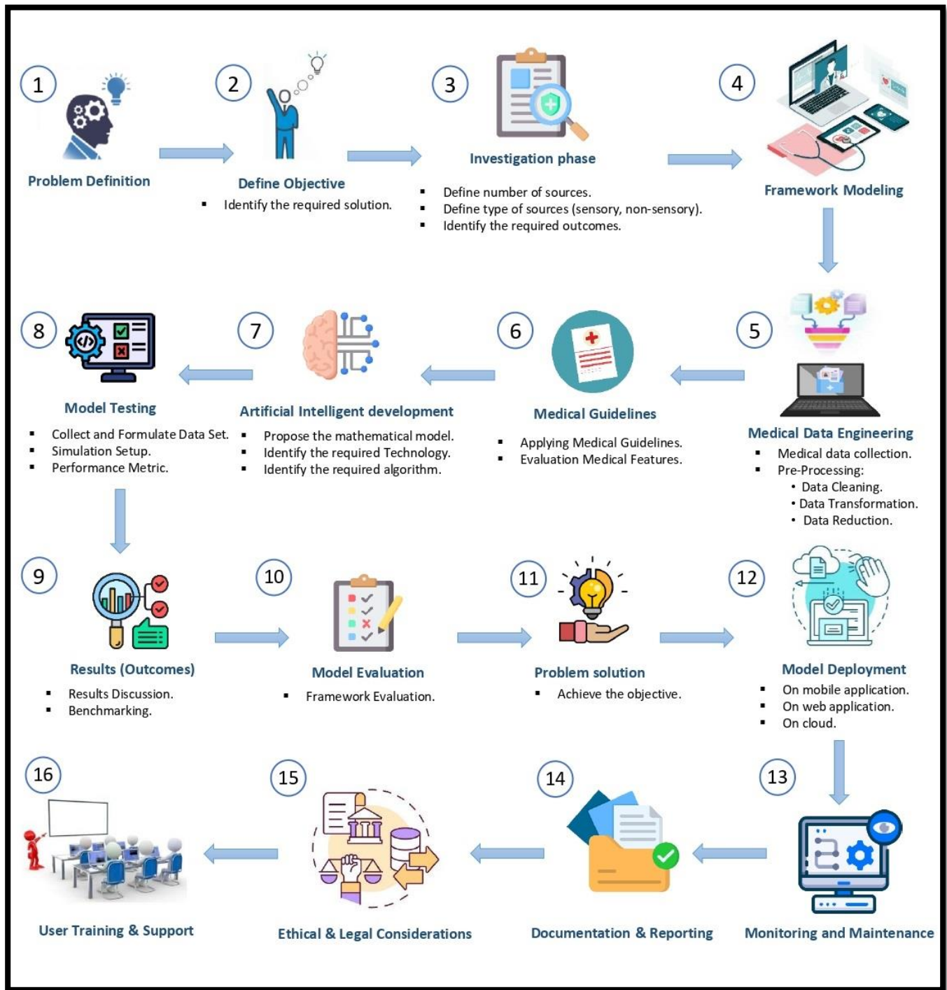
Fig. 2: Proposed Methodology
